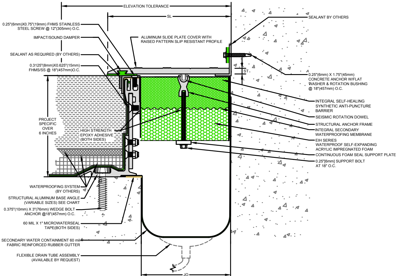
SSD Series Adjustable Height Expansion Joint (Slab-to-Column)
