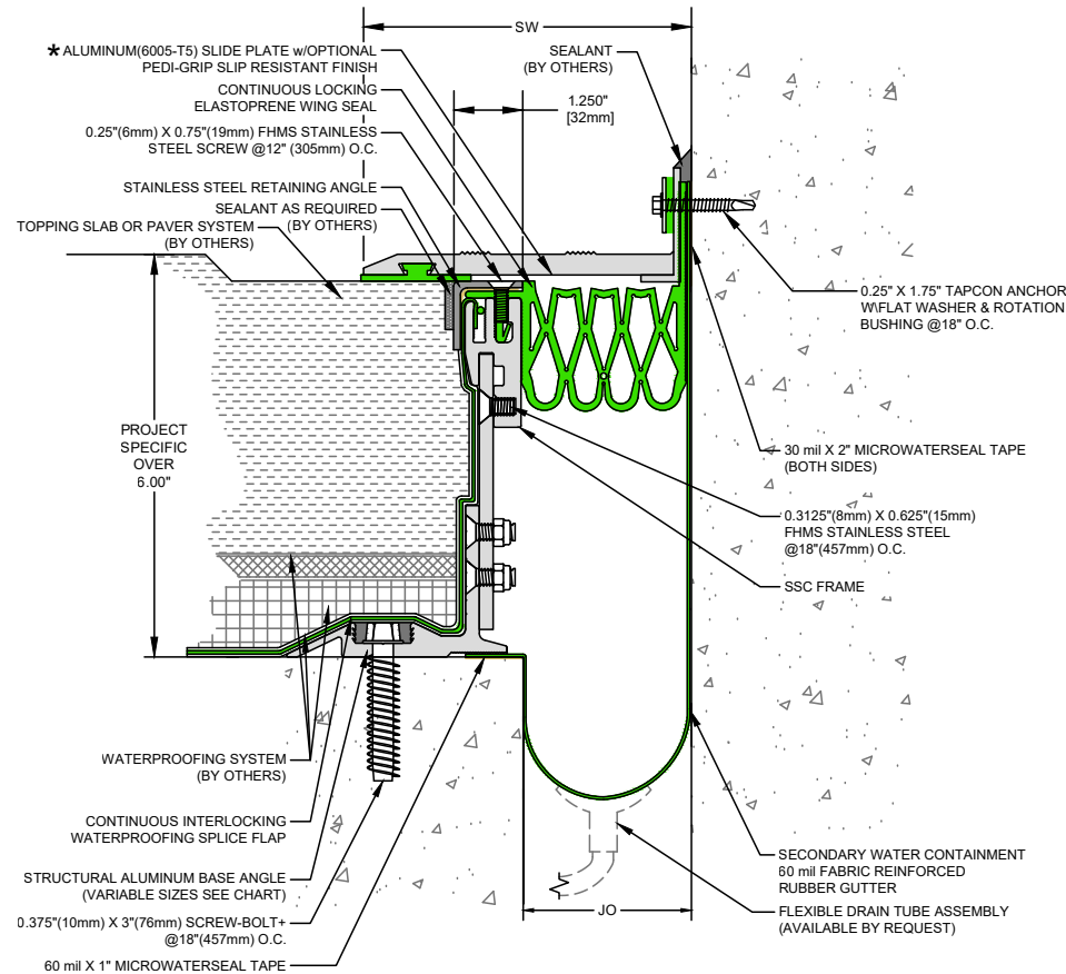
SSC Vehicular Series Adjustable Height Expansion Joint (Slab-to-Wall)
