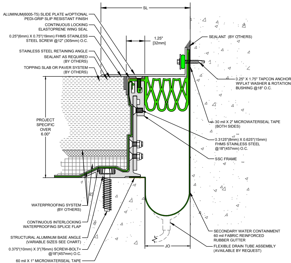
SSC Pedestrian Series Adjustable Height Expansion Joint (Slab-to-Wall)
