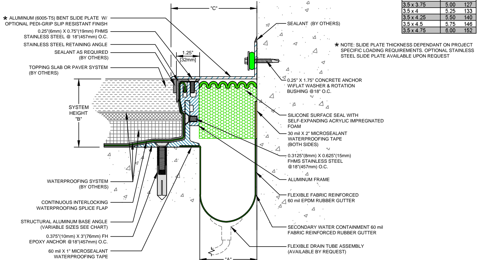
SCF SERIES EXPANSION JOINT (Slab-to-Wall)
