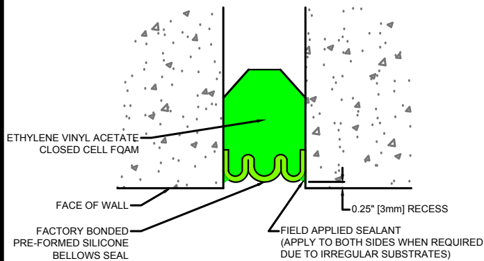
SCE Series Expansion Joint (Wall-to-Wall)
