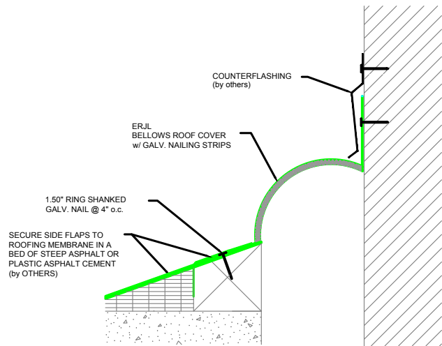
ERJL Series Expansion Joint (Roof-to-Corner)
