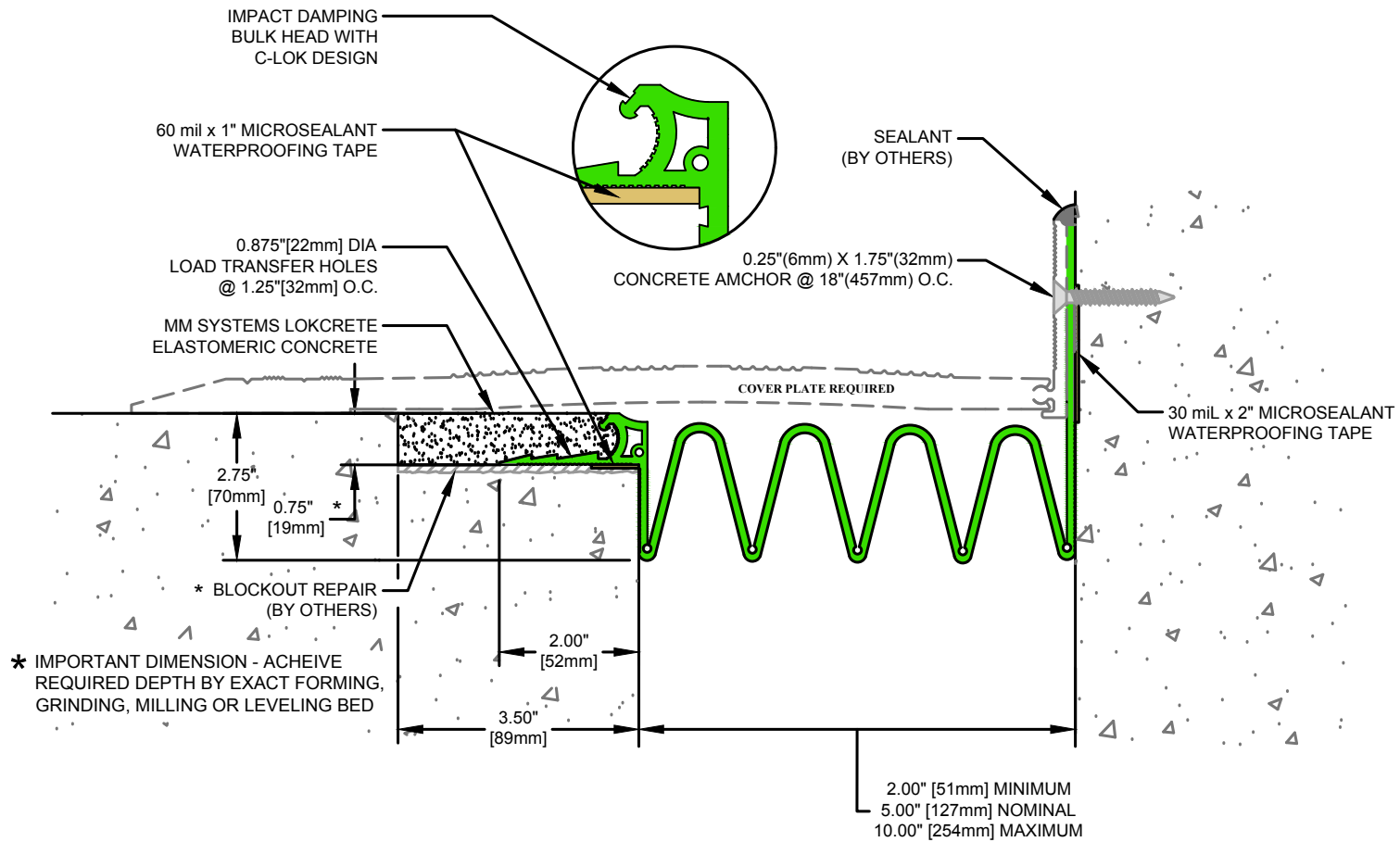
LSS-C-1600 SERIES EXPANSION JOINT (Slab-to-Wall)
