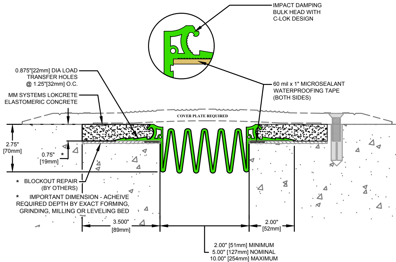
LSS-1600 SERIES EXPANSION JOINT (Slab-to-Slab)
