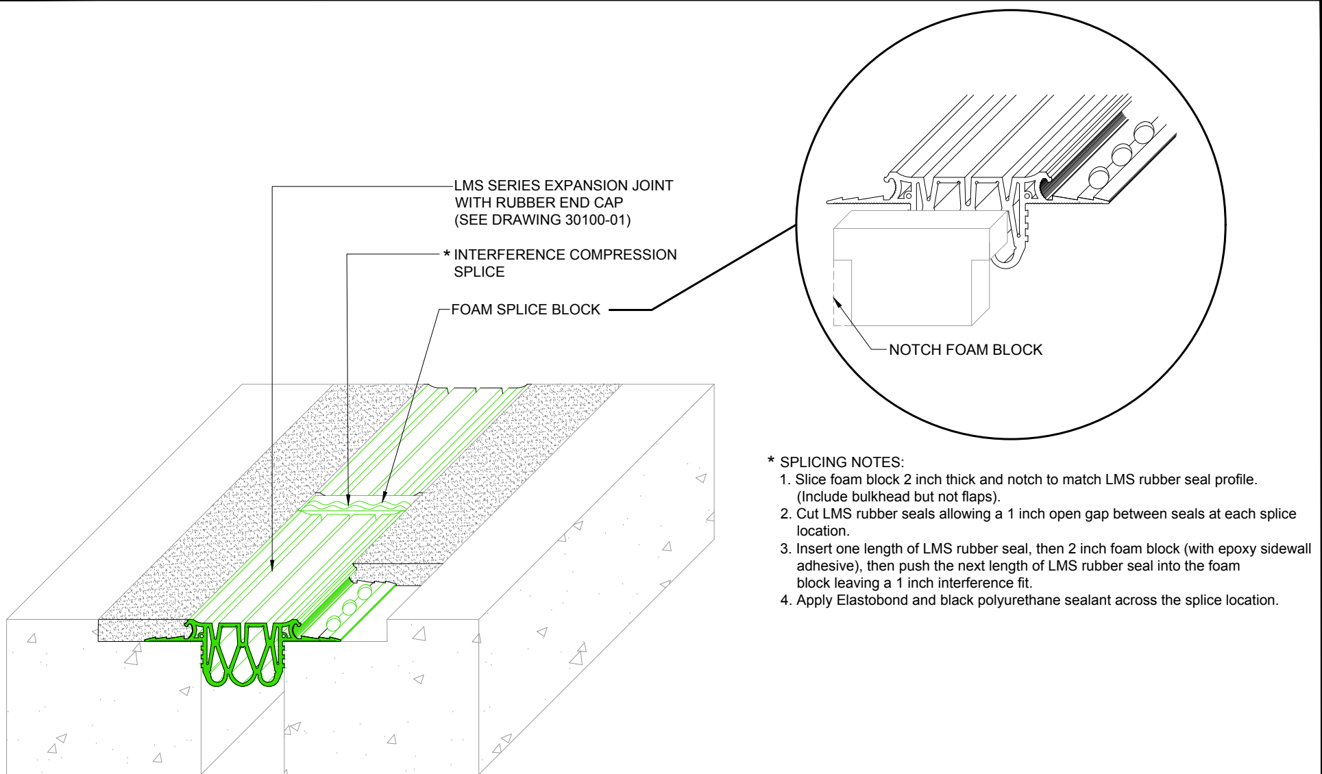
LMS Expansion Joint \ Seal Butt Splice Transition (Slab-to-Slab)
