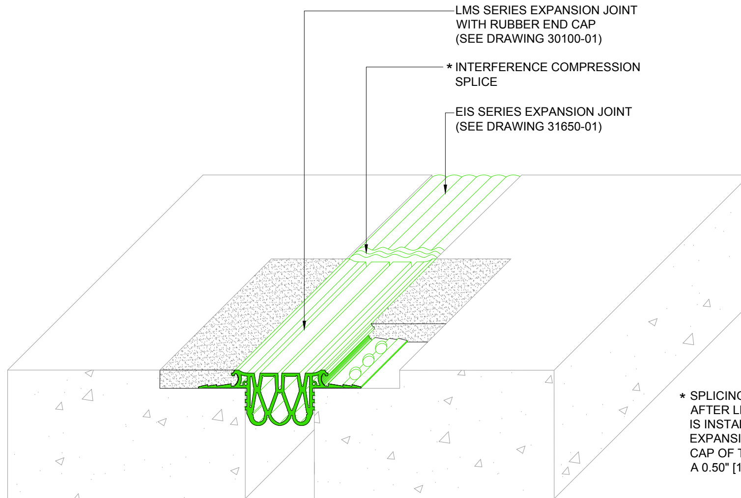
LMS-to-EIS Horizontal Butt Splice Expansion Joint Transition (Slab-to-Slab)
