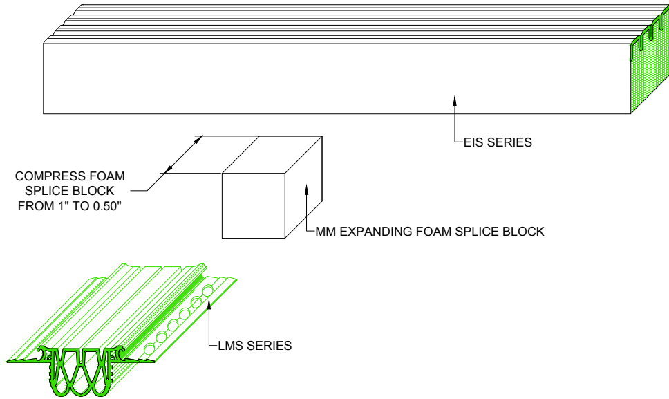
EXPLODED VIEW
