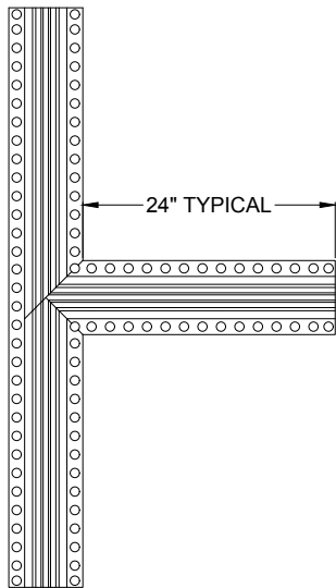
FACTORY "TEE" TRANSITION
