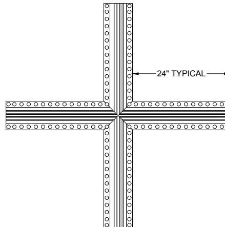
FACTORY "CROSS" TRANSITION
