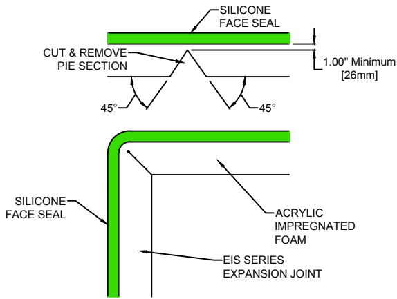
OUTSIDE CORNER MITER (SEE DRAWING 30751-01) DETAIL A
