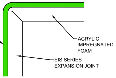
OUTSIDE CORNER MITER (SEE DRAWING 30751-01) DETAIL A
