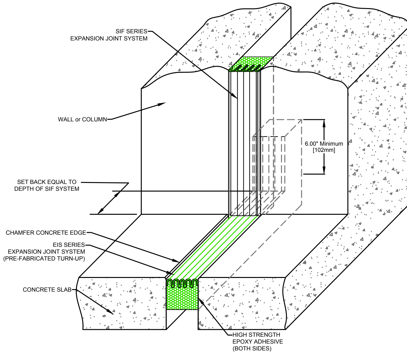
EIS-to-SIF Counterflash Transition (Slab-to-Wall Corner)
