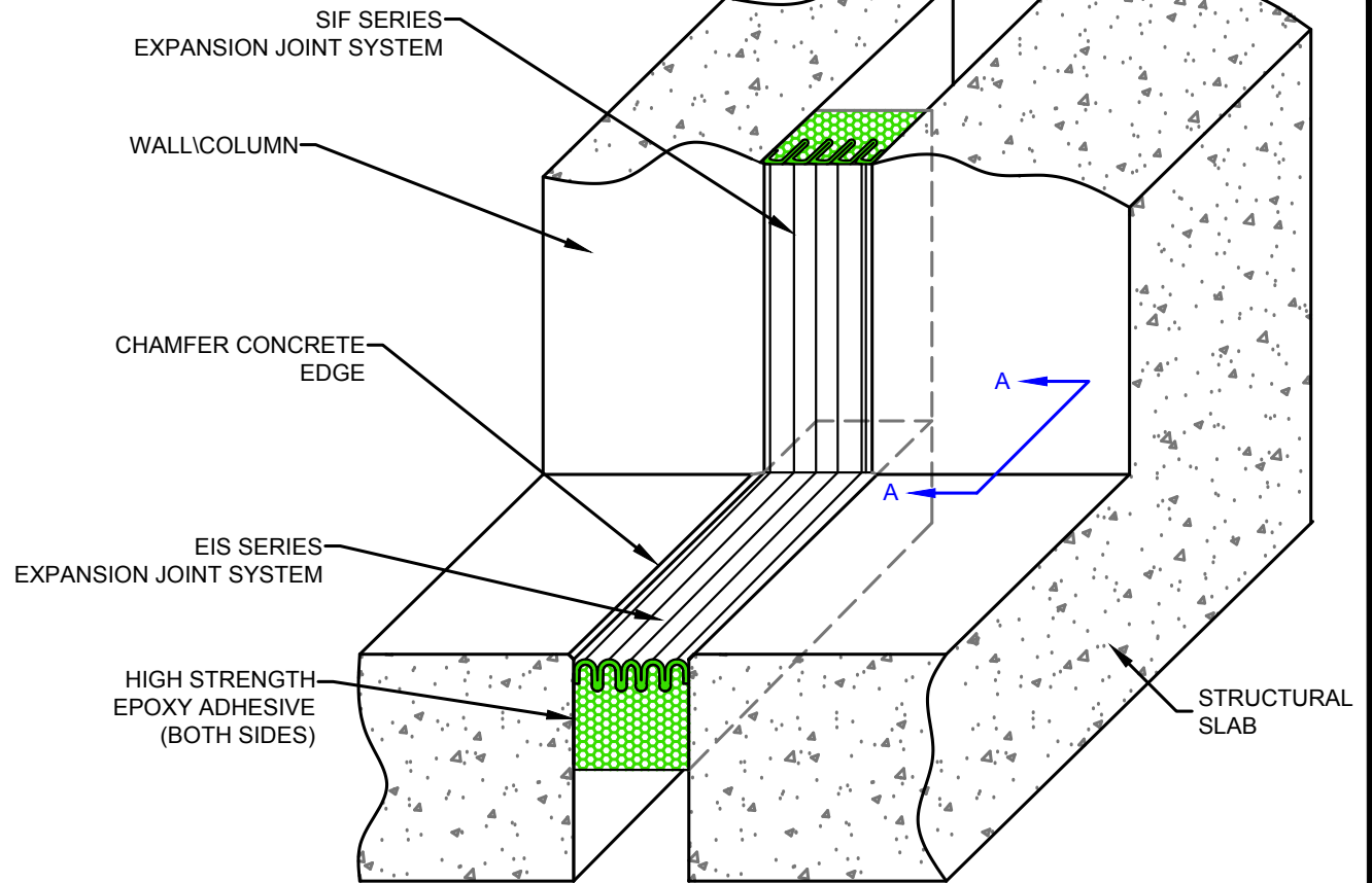
EIS-to-SIF Corner Transition (Slab-to-Wall Corner)
