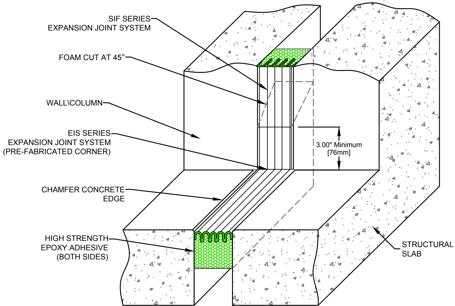
EIS-to-SIF Beveled Corner Transition (Slab-to-Wall Corner)
