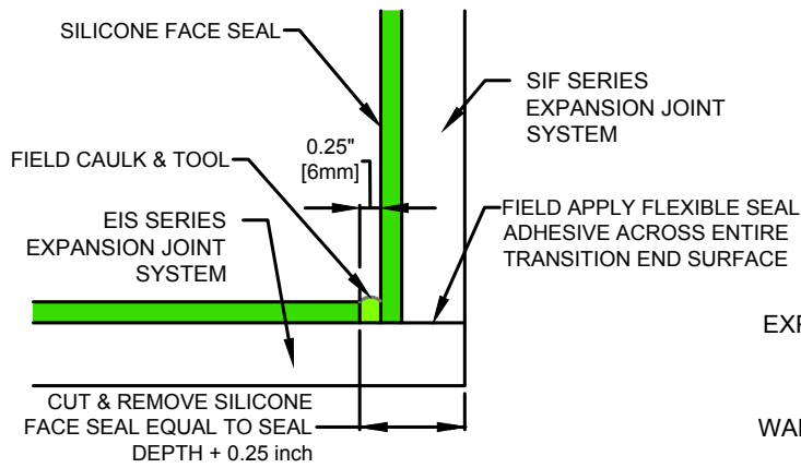
SECTION A-A (SEAL TRIM DETAIL)
