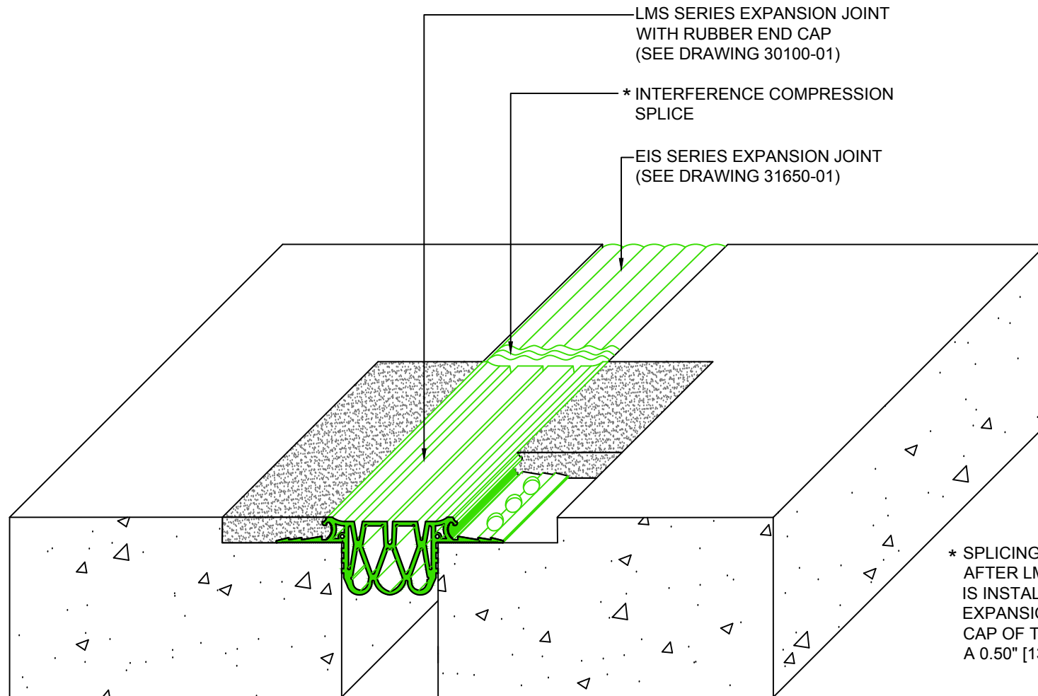
EIS-to-LMS Horizontal Butt Splice Expansion Joint Transition (Slab-to-Slab)
