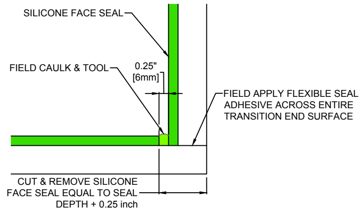
EIS SEAL TRIM DETAIL
