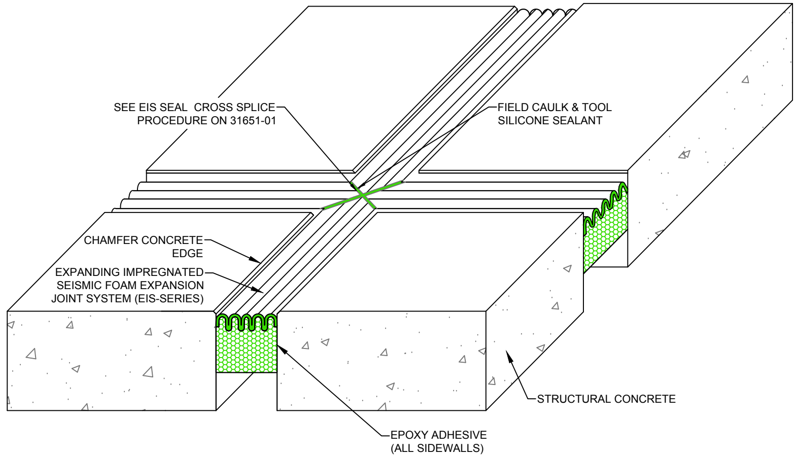
EIS Expansion Joint Cross Transition (Slab-to-Slab)
