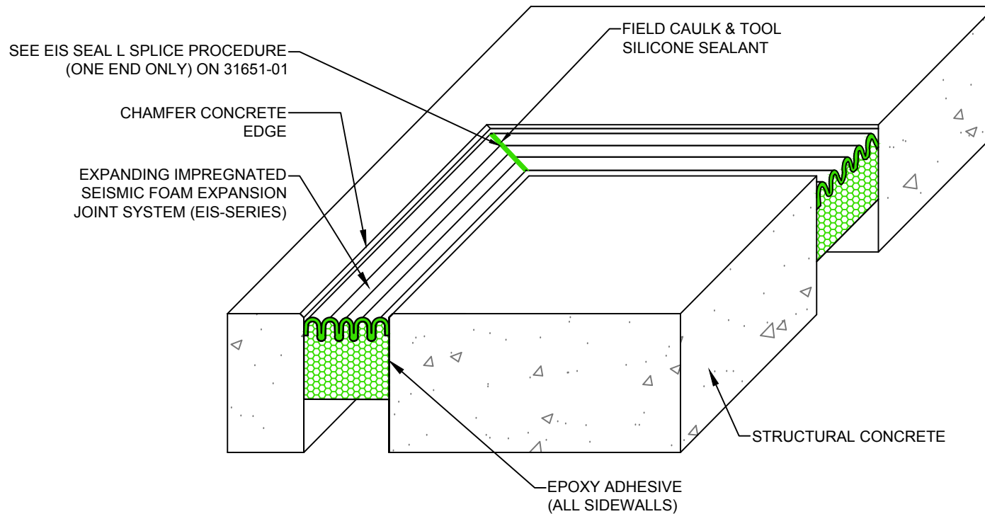
EIS Expansion Joint L Splice Transition (Slab-to-Slab)
