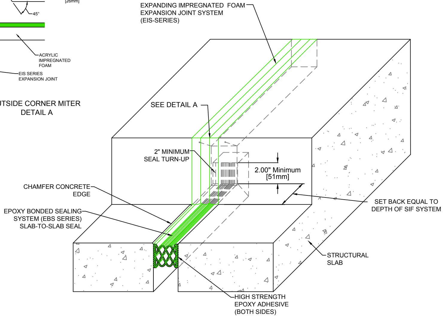
EBS-to-EIS Counterflash Expansion Joint Transition (Slab-to-Slab)
