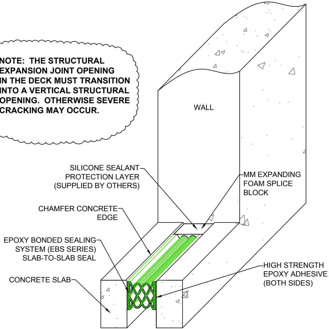
EBS End Termination Expansion Joint Transition (Slab-to-Slab)
