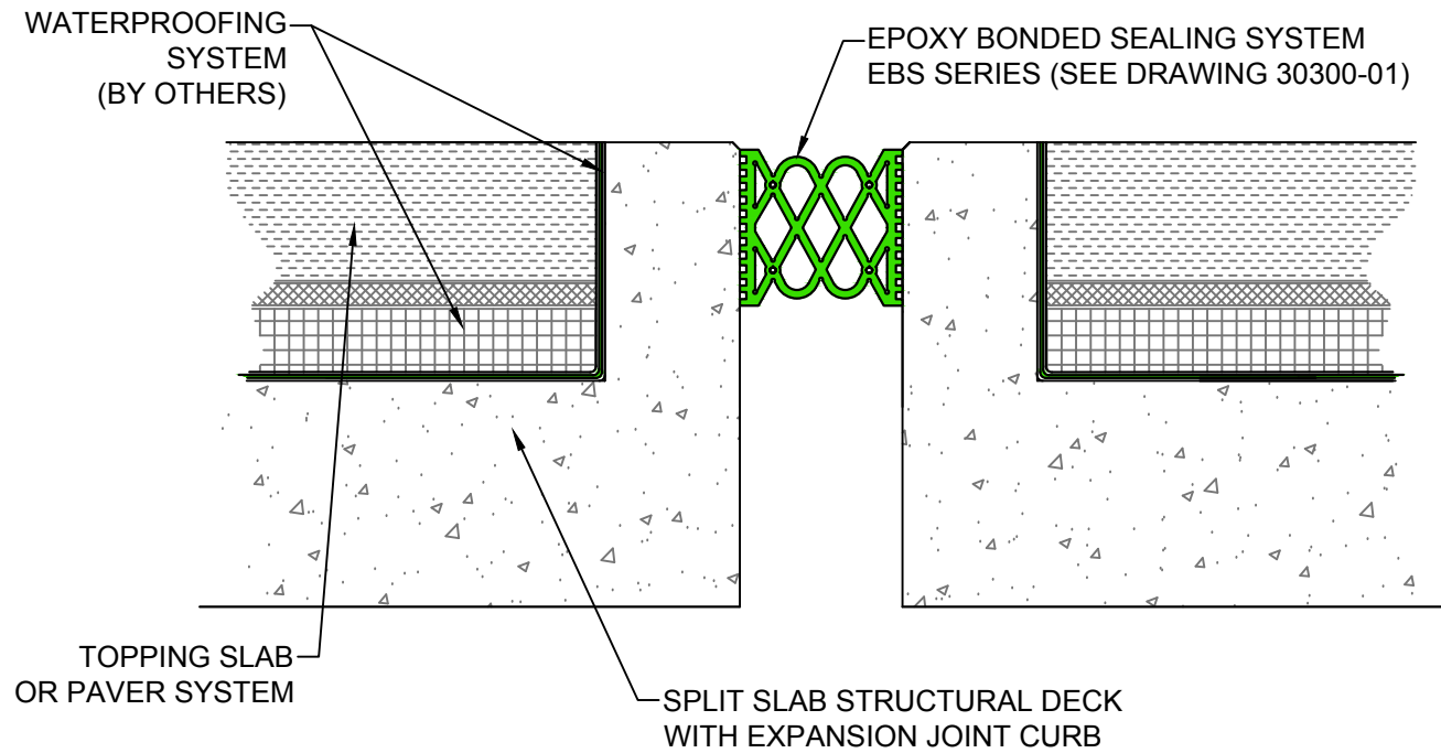
EBS Expansion Joint (Slab-to-Slab / Split Slab Plaza Deck)
