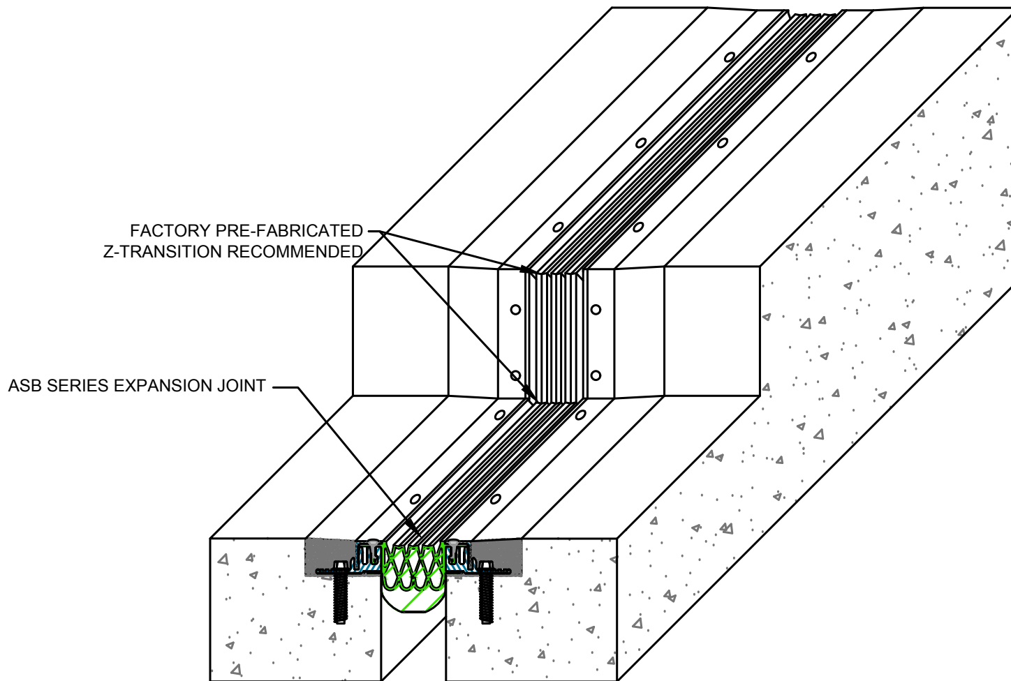
ASB Curb/Sidewalk Expansion Joint Transition (Curb Transition)
