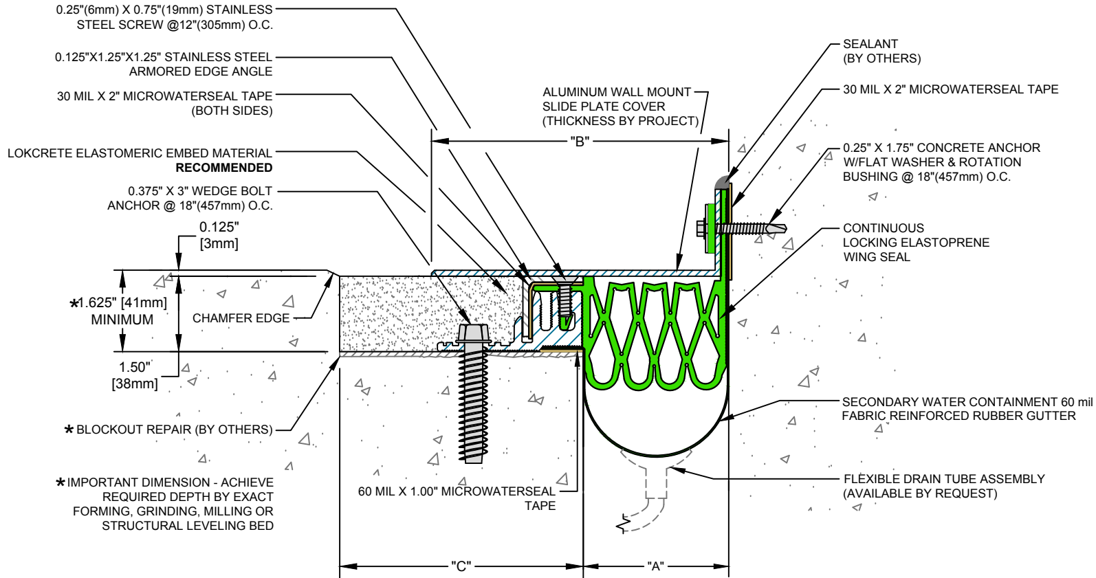
ABC Series Expansion Joint (Slab-to-Wall)
