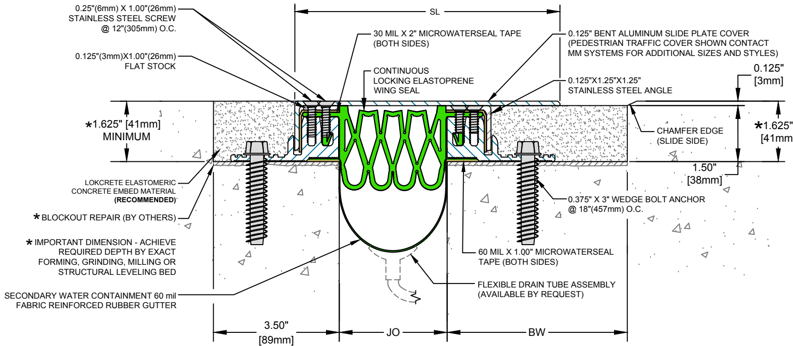
ABC Series Expansion Joint (Slab-to-Slab)
