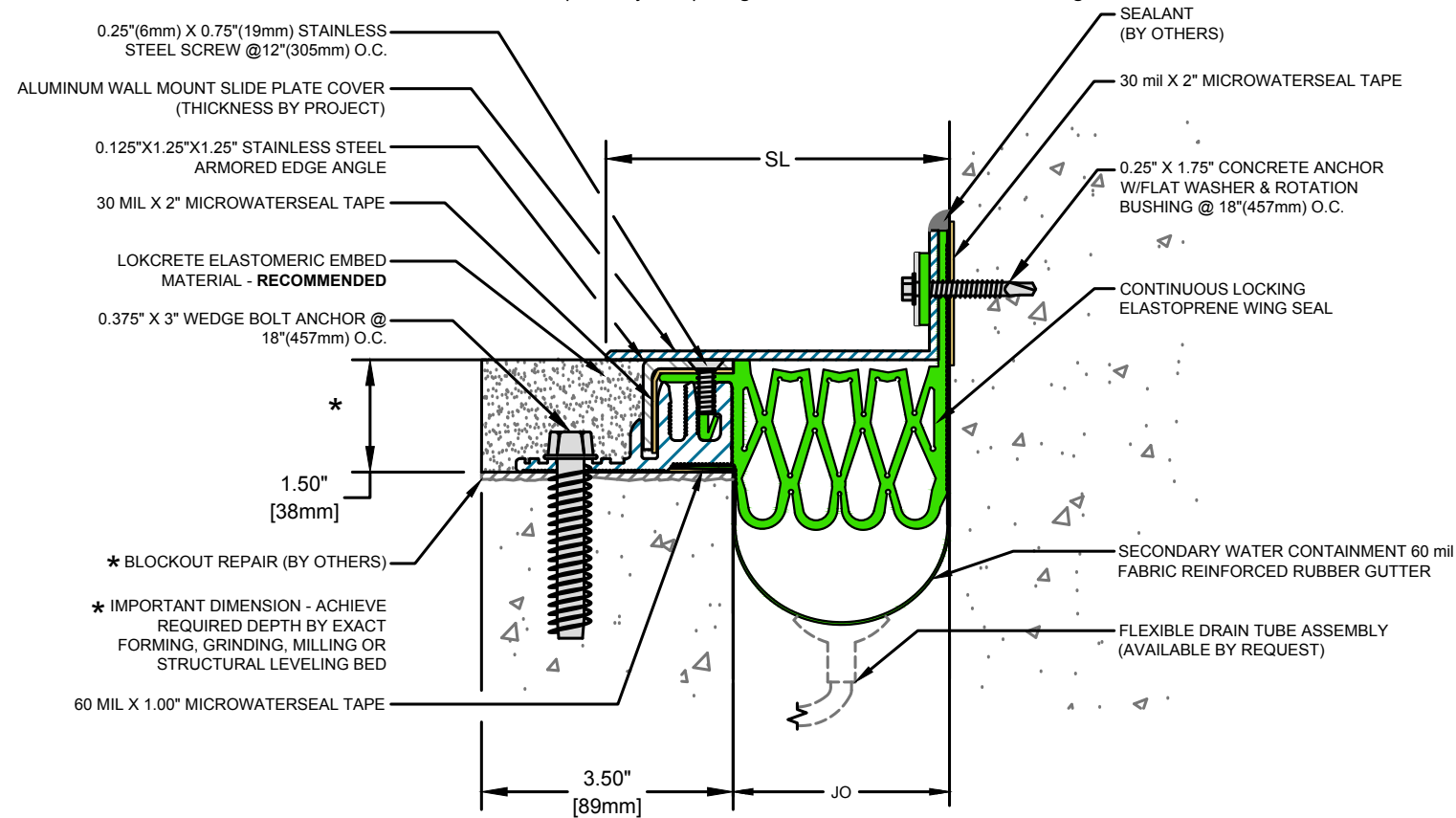
ABC Series Expansion Joint (Slab-to-Slab)
