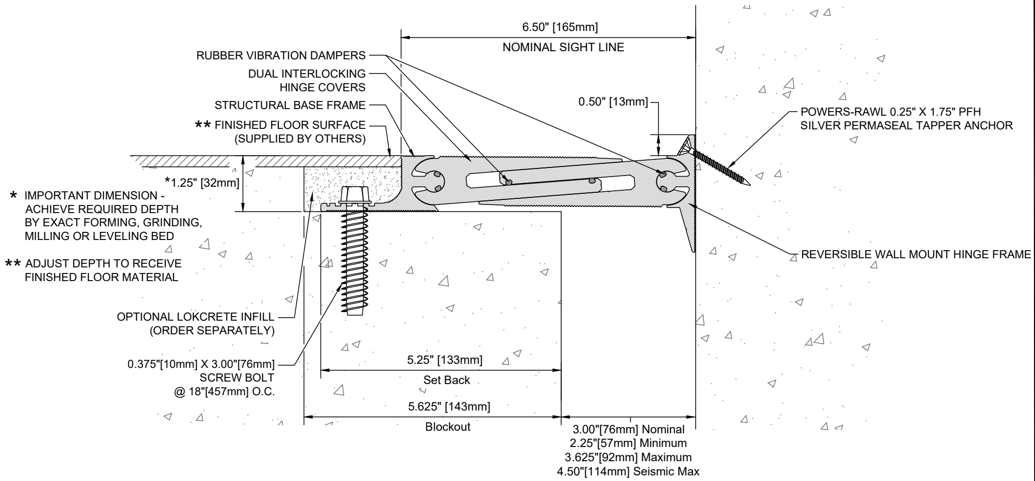
DIH-C-300 Expansion Joint (Floor-to-Wall / 0.50" Corner)
