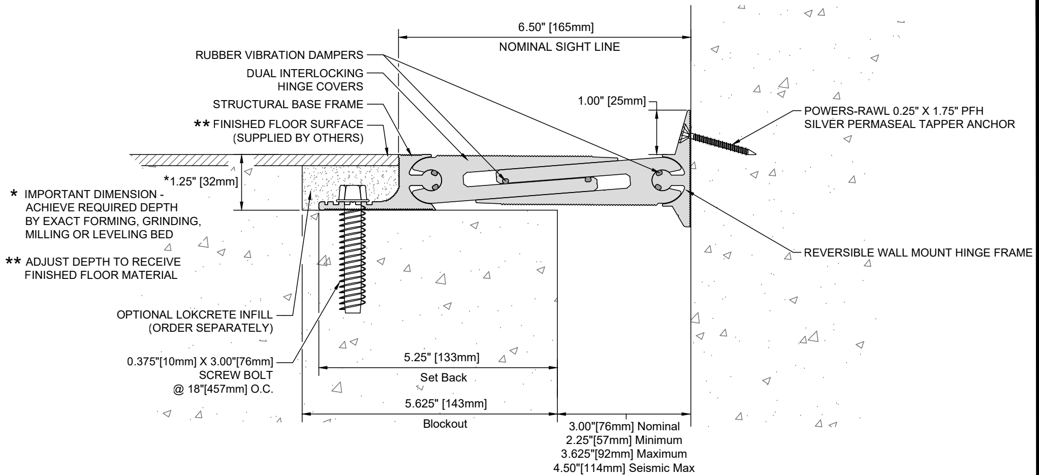
DIH-C-300 Expansion Joint (Floor-to-Wall / 1" Corner)
