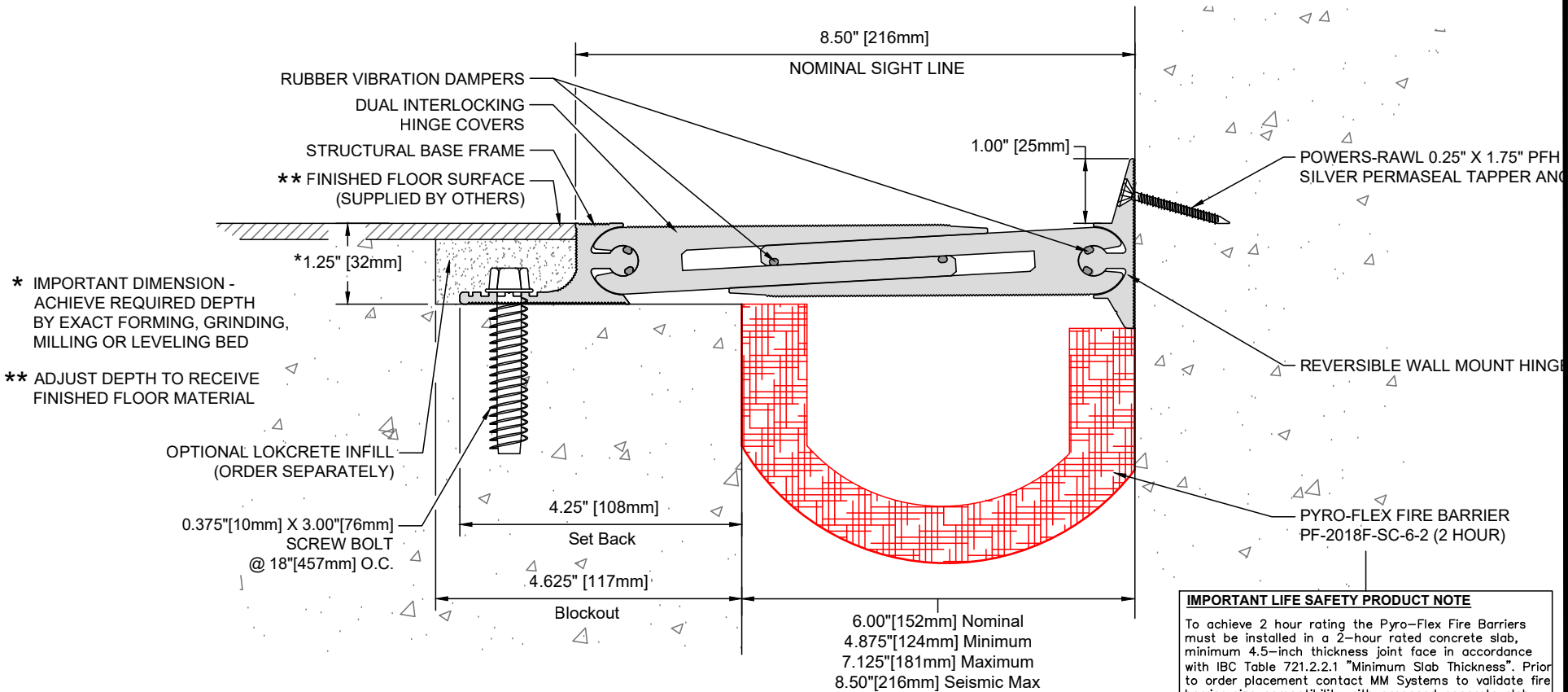
DIH-C-600-1.0 Fire Rated Expansion Joint (Floor-to-Wall / 1" Corner)
