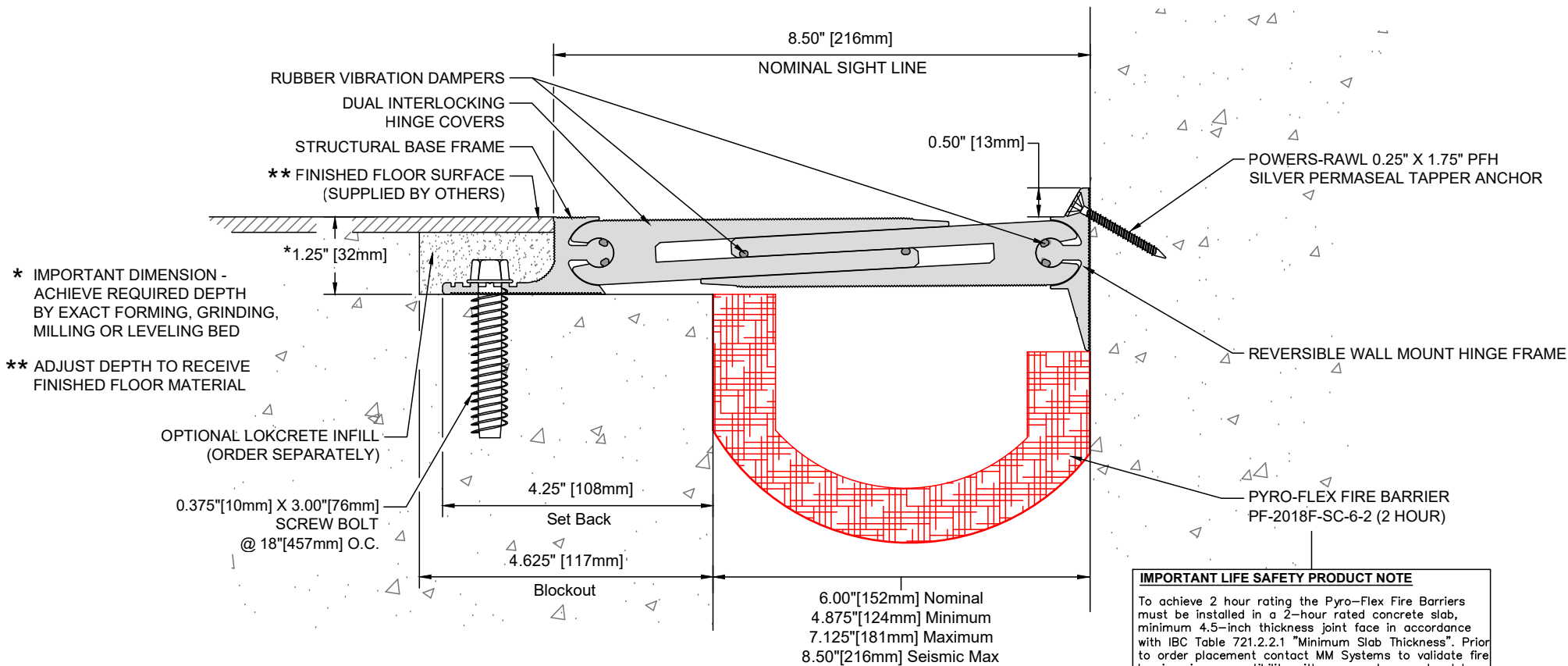
DIH-C-600-0.5 Fire Rated Expansion Joint (Floor-to-Wall / 0.50" Corner)
