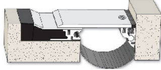
Model SSS-C Recessed/ Slab-to-Wall Movement 1.75" to 15"
