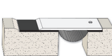
Model AID Slab-to-Slab / Movement 1.0" to 15.0"
