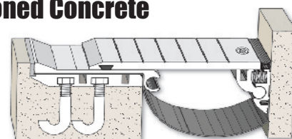
Model CIS-C Slab-to-Wall / Movement 2.5" to 12.5" Cast-In-Place Design
