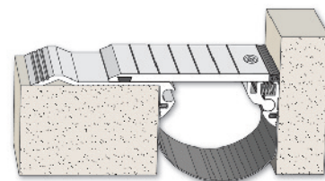
Model SMS-C Slab-to-Wall / Movement 2.0" to 12.5"
