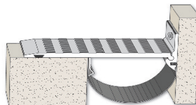
Model HSC-C Slab-to-Wall / Movement 1.0" to 15.0"
