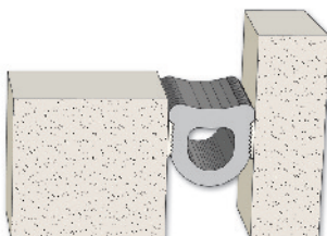
Model ERS Slab-to-Wall (Cover plate not required)
