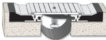
Model SSP Recessed/Slab-to-Slab Movement 1.0" to 18"
