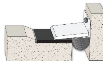
Model GID-C Slab-to-Wall / Movement 1.0" to 15.0"
