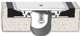
Model SNB Slab-to-Slab Thermal Movement Seismic Movement 18" Max.
