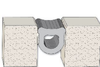
Model ERS Slab-to-Slab / Movement .5" to 3.75" (Cover Plate may be required - not shown)
