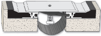
Model SSS Recessed/Slab-to-Slab Movement 1.0" to 18"
