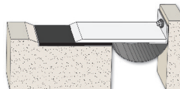
Model AID-C Slab-to-Wall / Movement 1.0" to 15.0"
