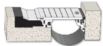
Model SSP-C Recessed/Slab-to-Wall Movement 1.75" to 15"
