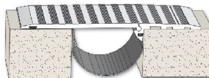
Model HSC Slab-to-Slab / Movement 1.0" to 15.0"
