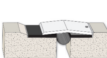
Model GID Slab-to-Slab / Movement 1.0" to 15.0"
