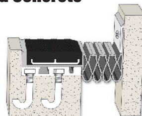
Model EMC-C / Cast-In Slab-to-Wall / Movement .75" to 6.5"
